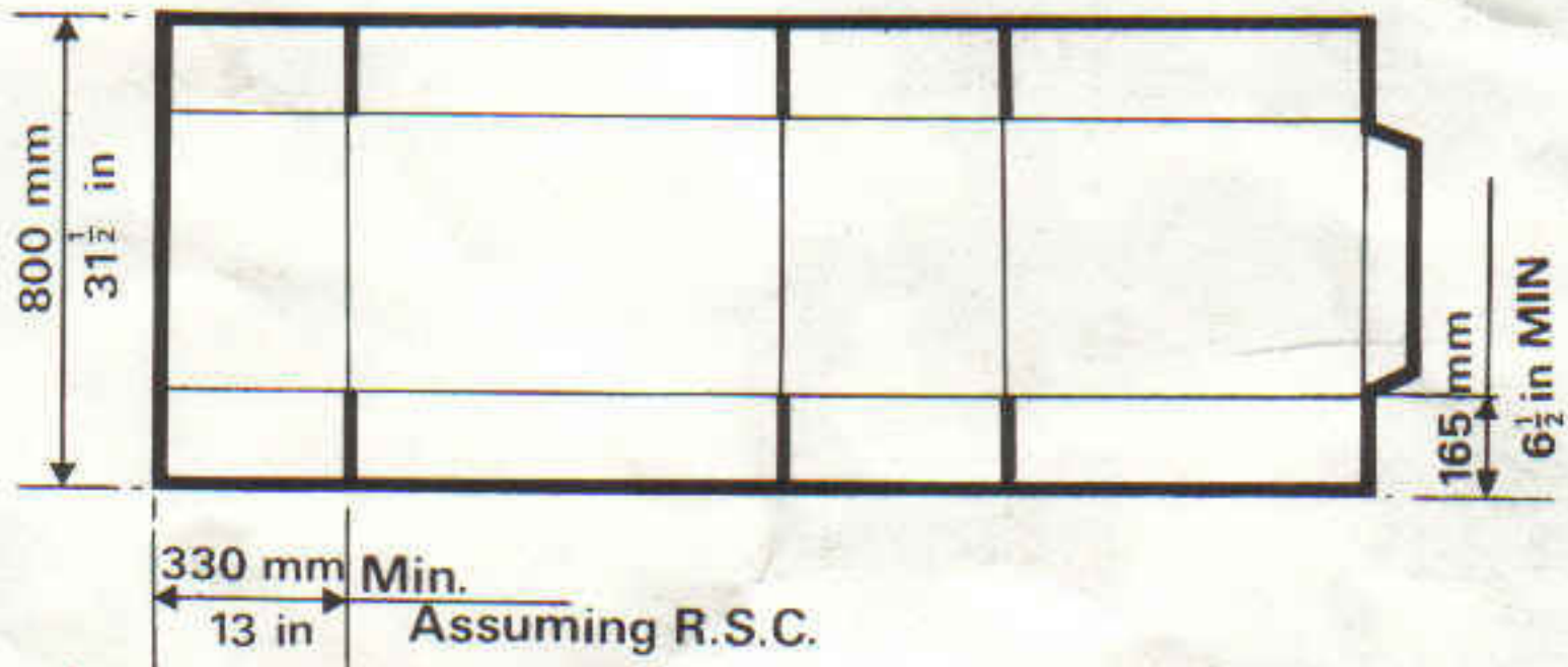
Maximum skip fed box with minimum end panel
