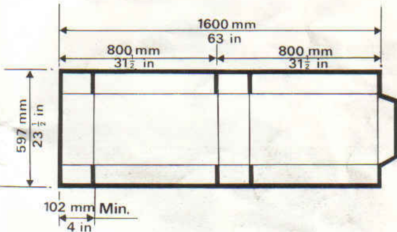
Maximum box with minimum end panel
