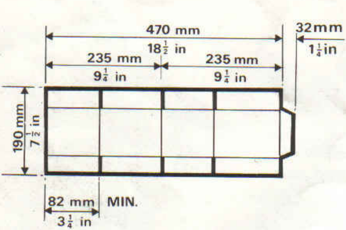
Minimum box with minimum end panel
